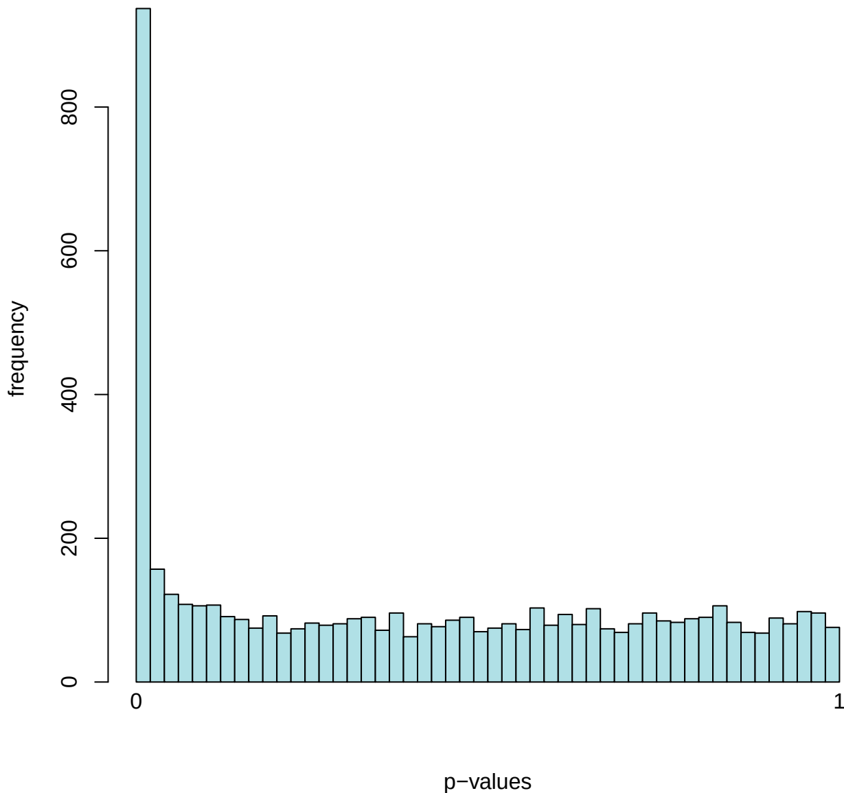
Histogram of p-values for Sample_Variance: Mutant vs Wildtype
