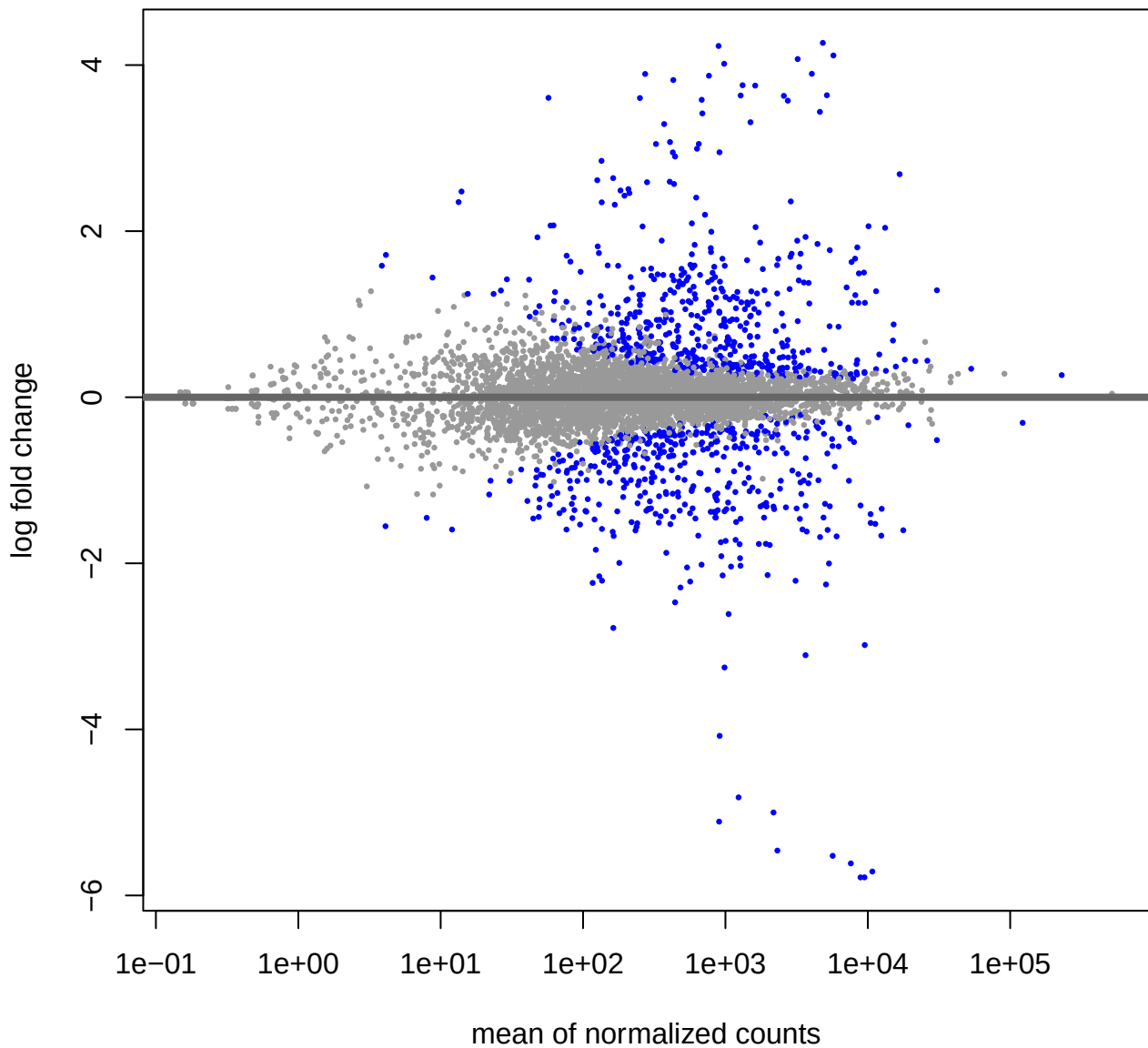
MA-plot for Sample_Variance: Mutant vs Wildtype
